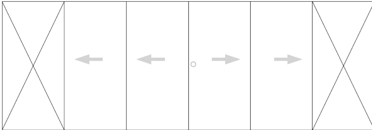
Central opening sliding (6 sheets, 3 rails)
