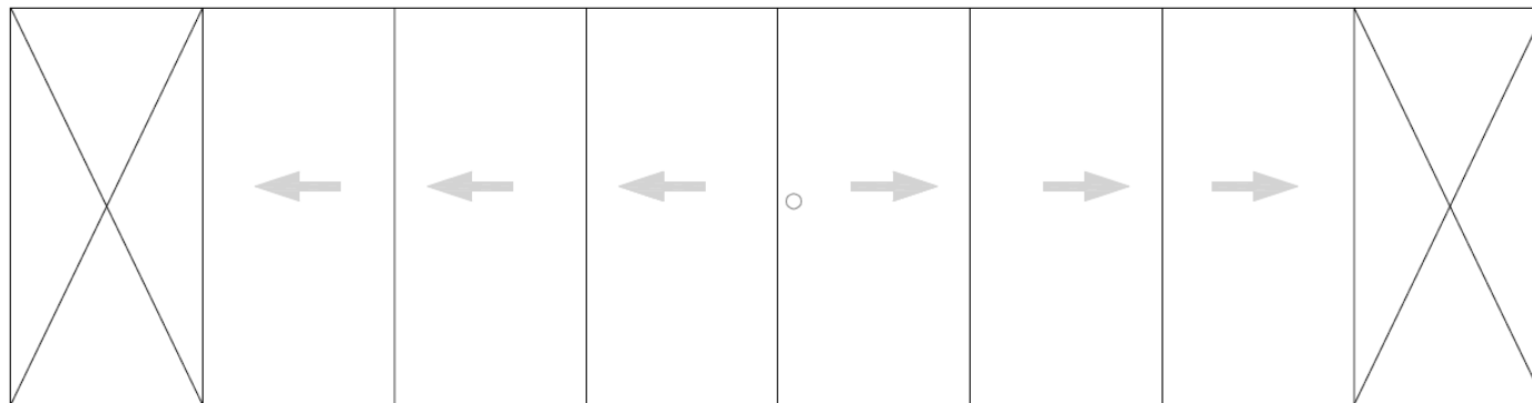
Central opening sliding (8 sheets, 4 rails)
