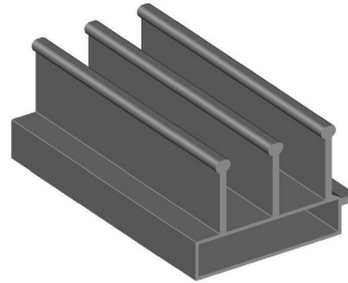
PR021- UPPER GLASS FRAME GLASS SLIDING 5+5 REF:37162
