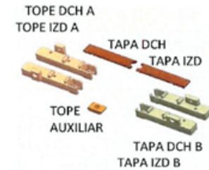
PR017- AB GLASS SLIDING AUXILIARY STOP
